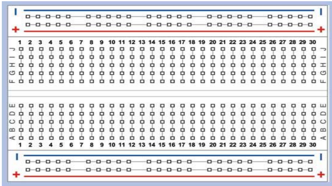
Figure 1. Breadboard connection example 1. [Ref. Internet]
