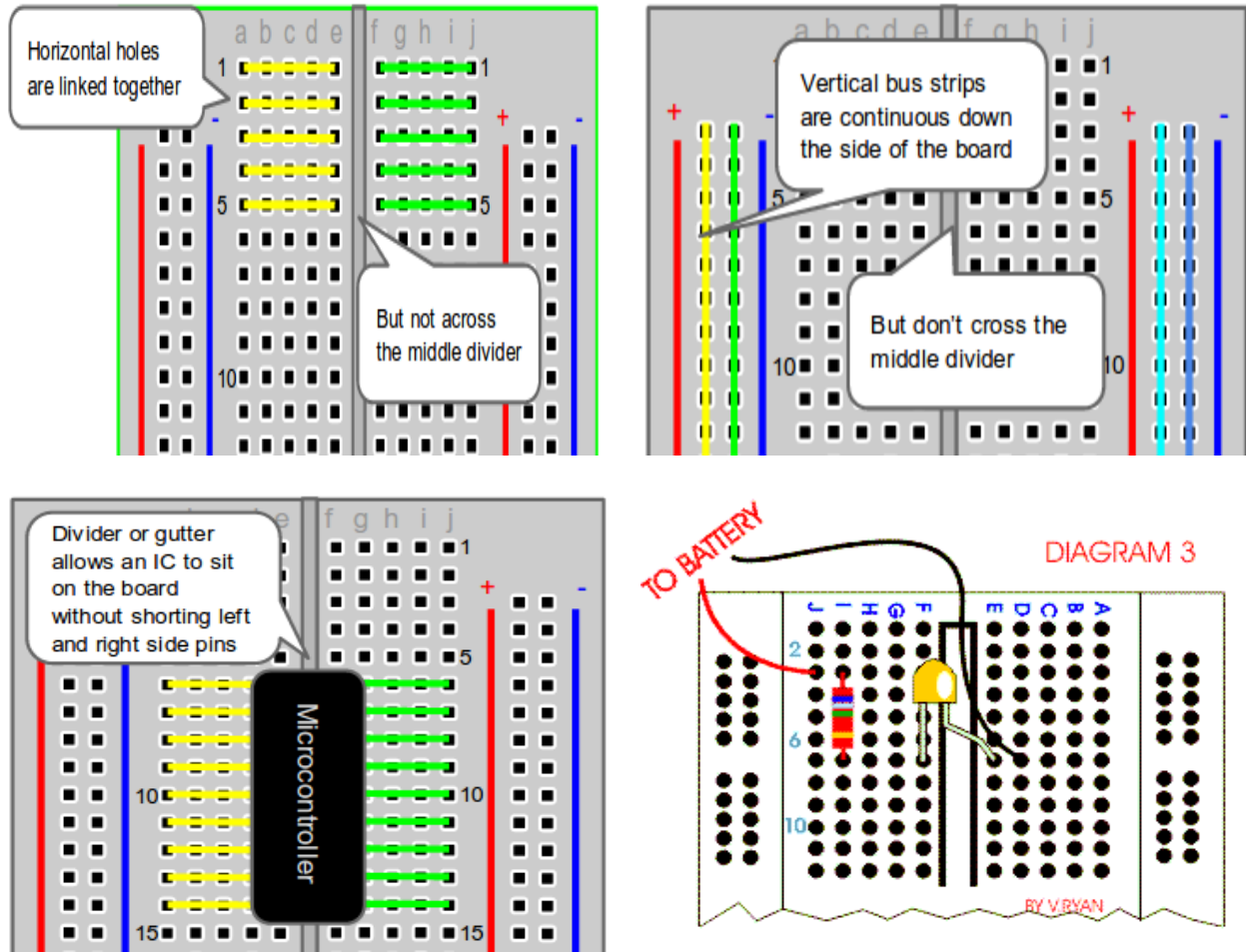
Figure 3. Breadboard connection example 3. [Ref. Internet]
