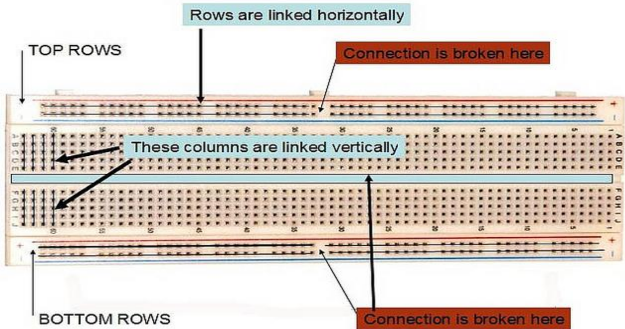
Figure 2. Breadboard connection example 2. [Ref. Internet]
